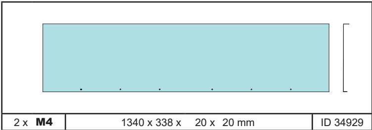
1 x M2 1340 x 338 x 30 x 20 mm ID 36571
