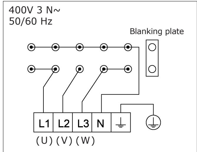
Wiring diagram for Durano / Durano Black sauna heater with 7.5 kW
