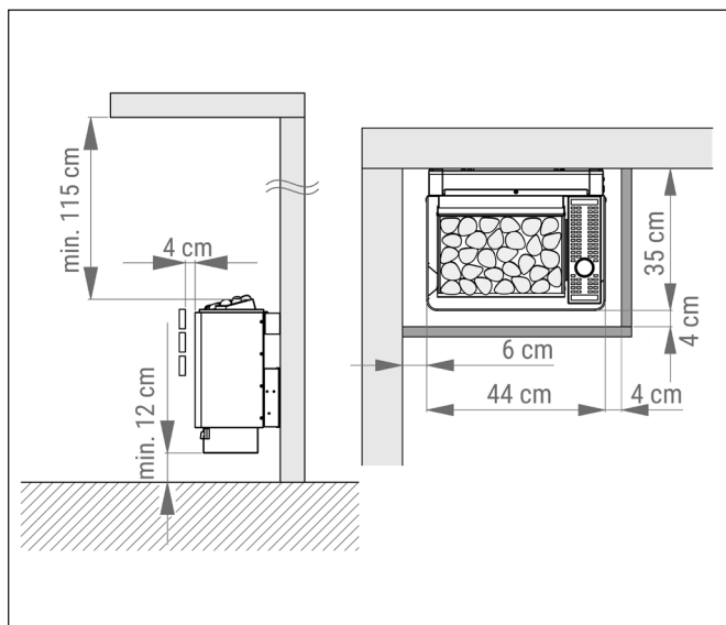
Fig. 1 - Minimum distances
