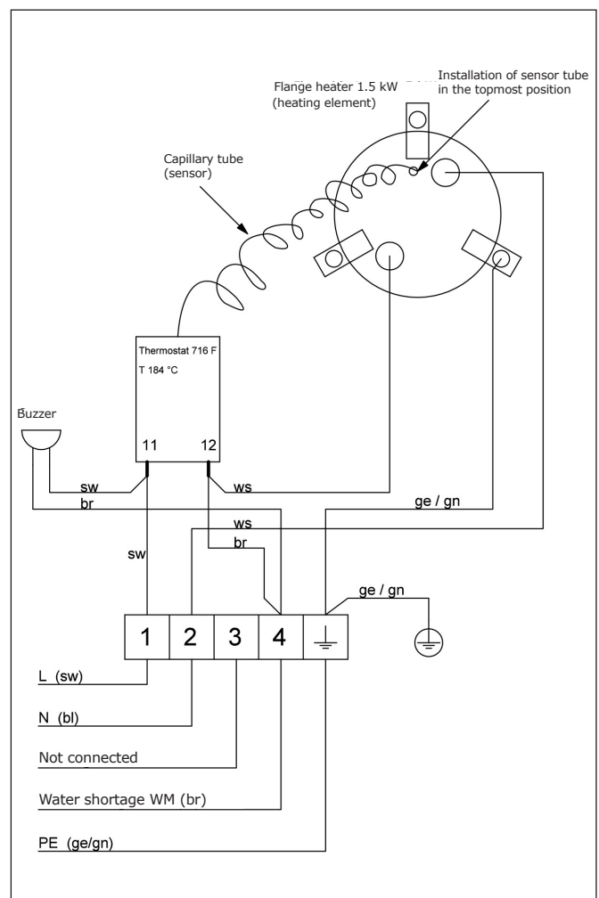
Wiring diagram for steamer
