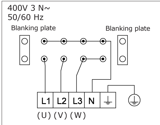
Wiring diagram for Durano sauna heater with 6.0 kW
