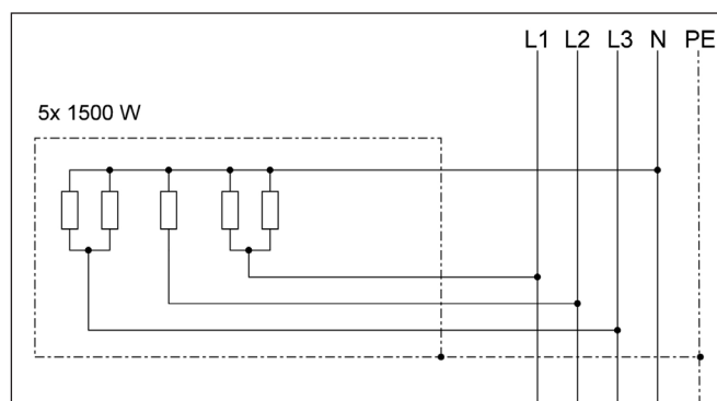
Durano / Durano Black sauna heater with 7.5 kW
