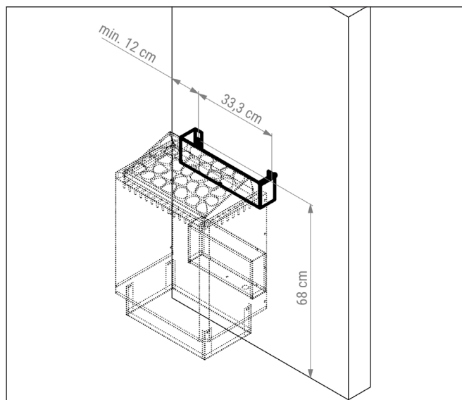
Fig. 2 - Wall mounting installation
