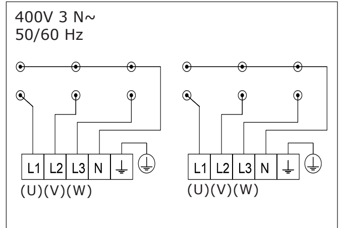
Connection diagram for Ferro sauna heater – 12.0 kW (dual-circuit) with PE
