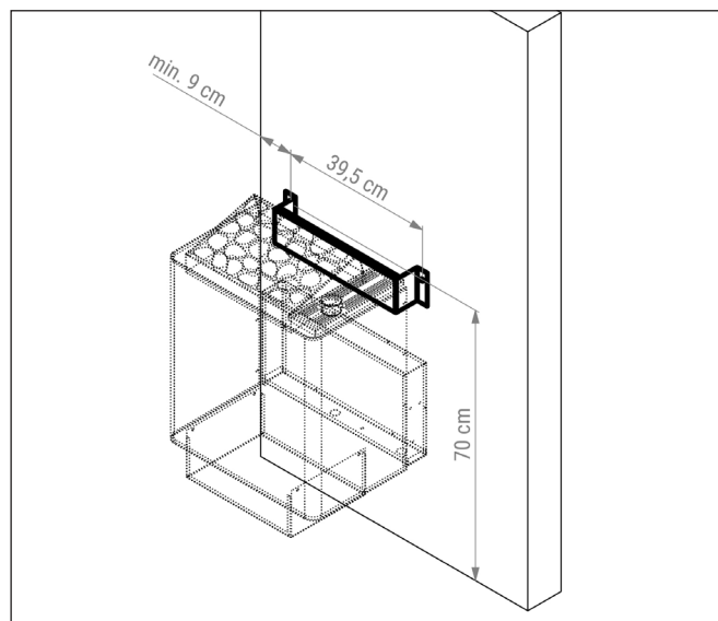
Fig. 2 - Wall mount bracket installation
