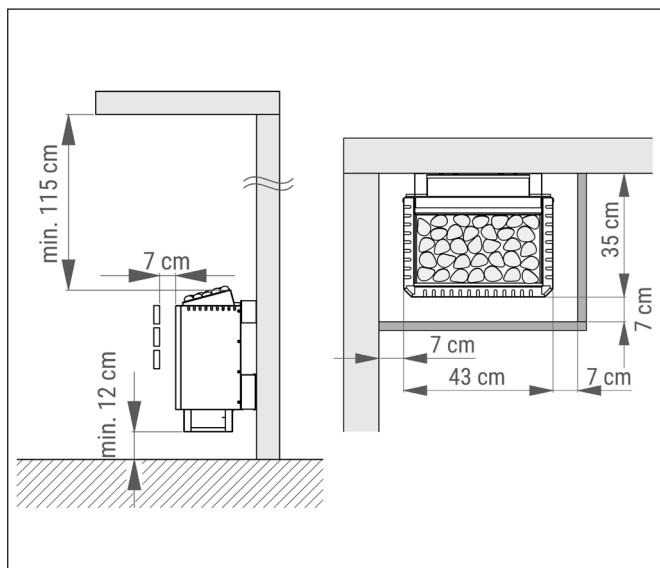
Fig. 1 - Safety distances
