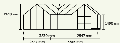
ICON GARDENHOUSE 8 · 13,0 m 2 (8' x 12')
