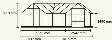
ICON GARDENHOUSE 8 · 13,0 m 2 (8' x 12')
